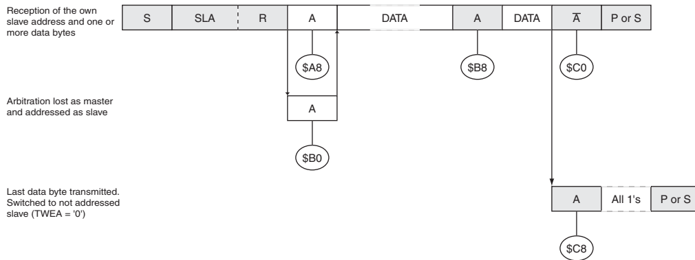
Figure 22-18. Formats and States in the Slave Transmitter Mode
