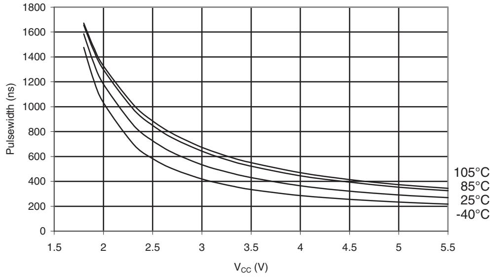
Figure 34-48. ATmega168PA: Minimum Reset Pulse Width vs. Vcc
