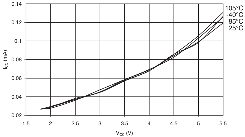
Figure 34-3. ATmega168PA: Active Supply Current vs. V_{CC} (Internal RC Oscillator, 128kHz)
